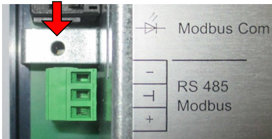
Figure 2: Communication indicator (LED) of the Modbus communication interface of the reactive power controller CX plus
